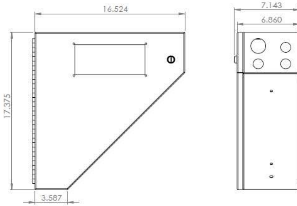
Figure 24: Controller box and UPS dimensions
