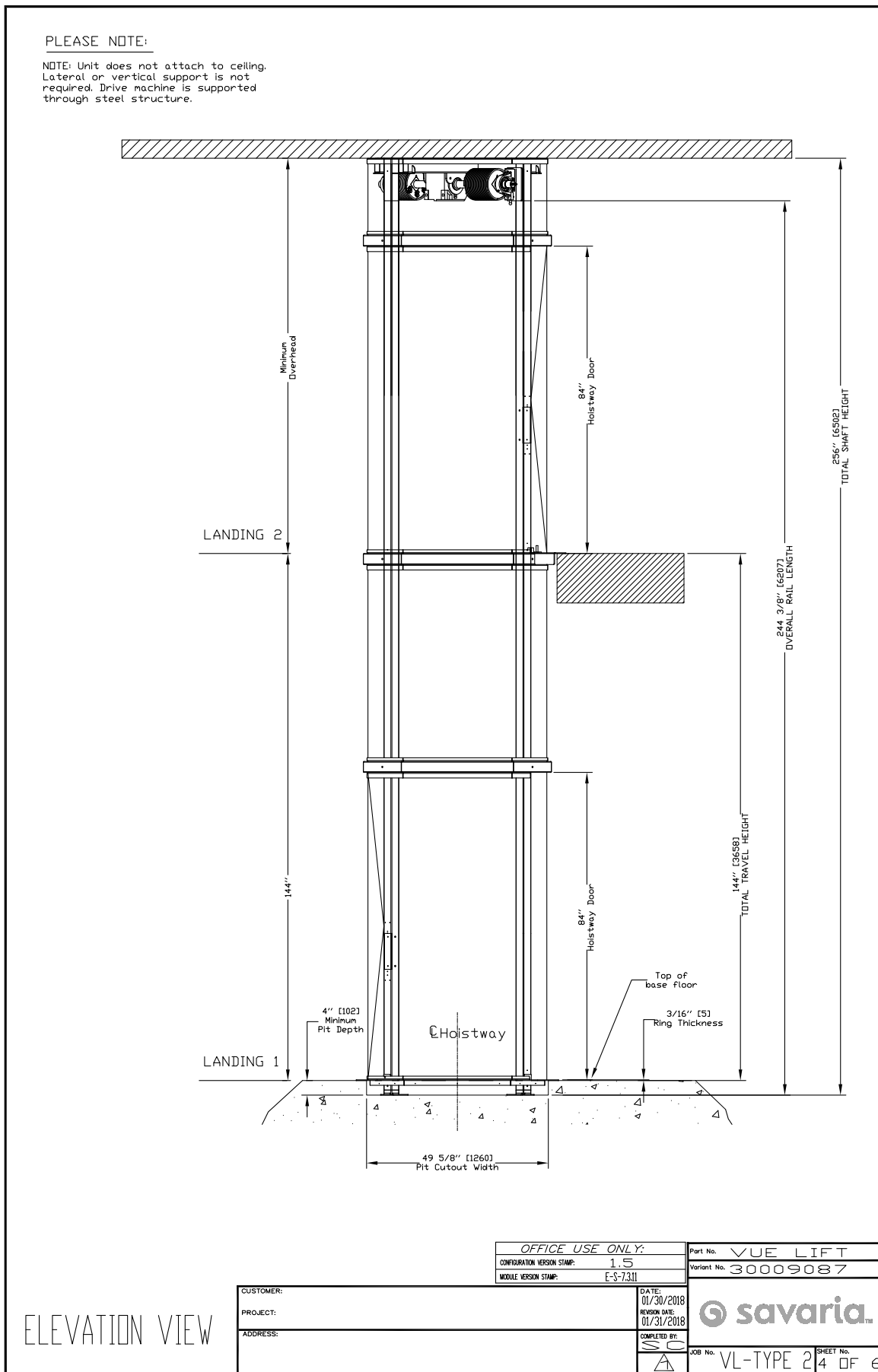
Figure 20: Elevation view (octagonal glass, type 2)
