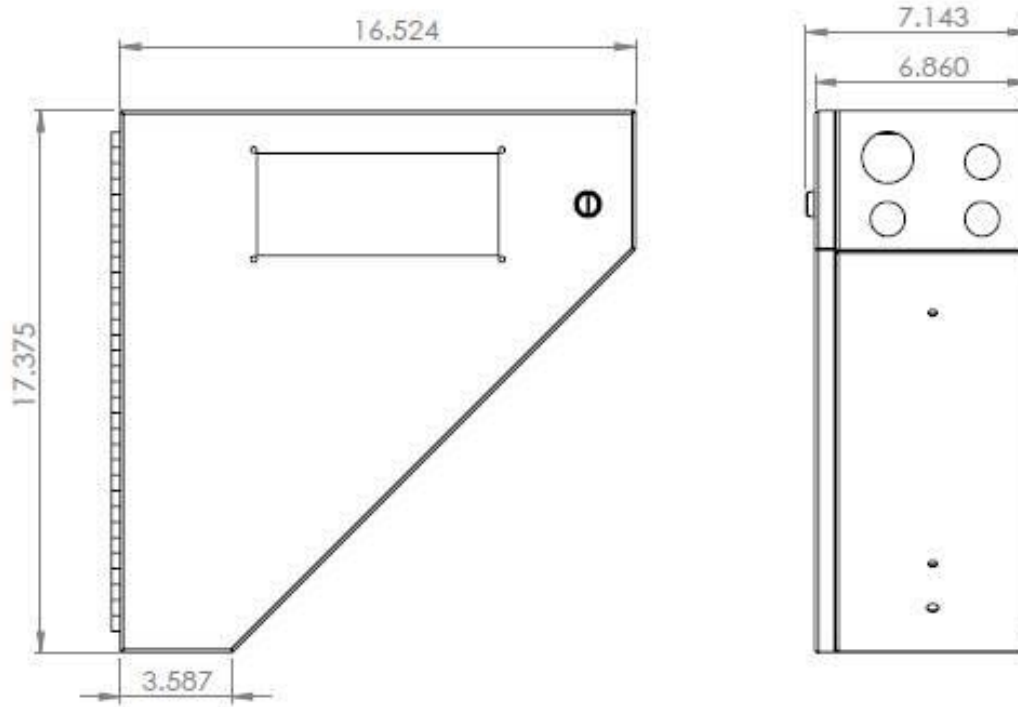
Figure 9: Controller box and UPS dimensions
