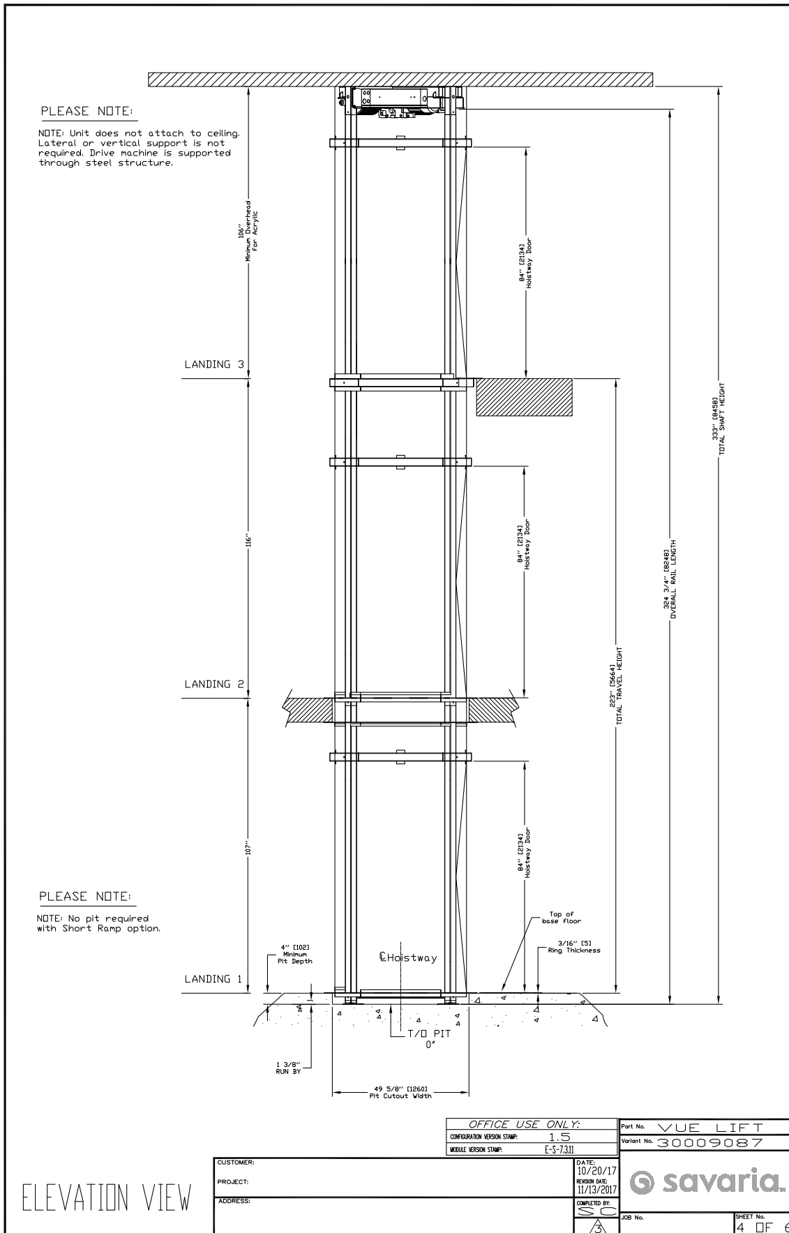
Figure 14: Elevation view (octagonal, type 1)
