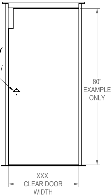
HOUSE VIEW WITH "L" BRACKET STOPPER
